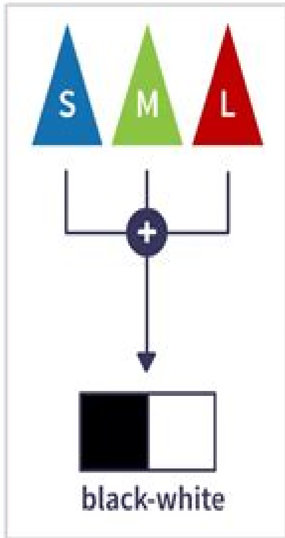
Achromatic System
