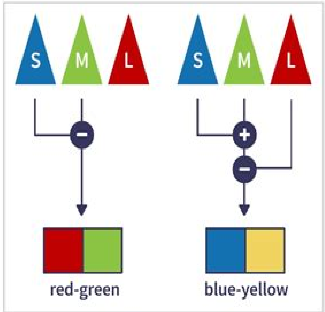
Chromatic System
